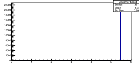
Lossed Energy in carrier board at Alpha (d = 29mm)
