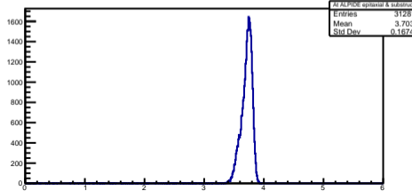
Lossed Energy in ALPIDE epitaxial + substruct at Alpha (d = 29mm)
