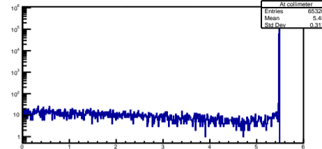
Lossed Energy in collimeter at Alpha (d = 29mm)
