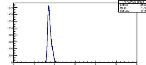
Lossed Energy in ALPIDE circuit at Alpha (d = 29mm)
